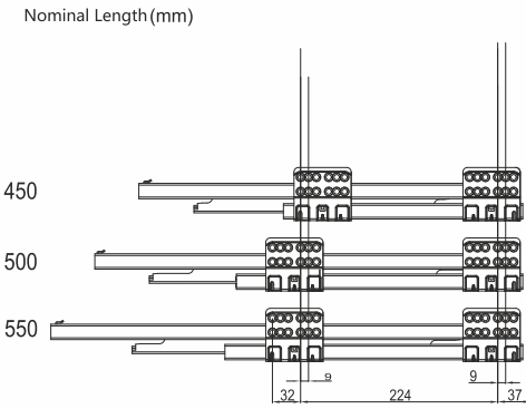
The drawer runners mounting dimensions
