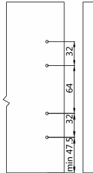
Inserta & General Panel Mounting hole size
