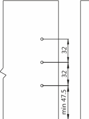
Inserta & General Panel Mounting hole size
