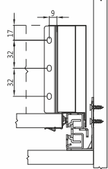
Mounting Dimensions for the back plate
