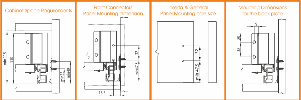
The drawer runners mounting dimensions
