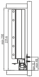
Cabinet Space Requirements
