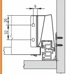
Mounting Dimensions for the back plate
