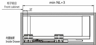
Cutting Dimensions for 16mm - thick MDF
