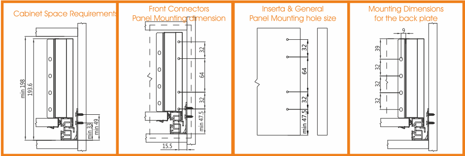
The drawer runners mounting dimensions
