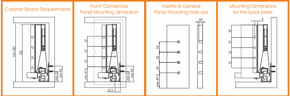
The cabinet body rail mounting dimensions
