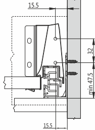
Front Connectors Panel Mounting dimension
