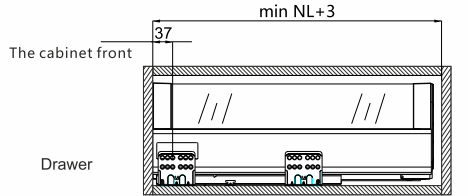
Cutting Dimensions for 16mm - thick MDF
