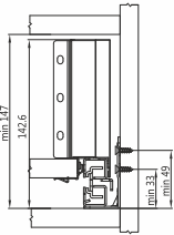
Cabinet Space Requirements
