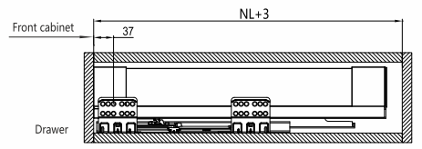
Cutting Dimensions for 16mm - thick MDF
