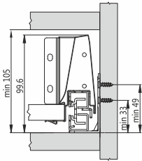
Cabinet Space Requirements
