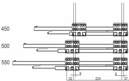
Cutting Dimensions for 16mm - thick MDF
