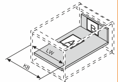
Cutting Dimensions for 16mm - thick MDF
