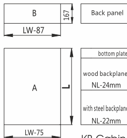
Cutting Dimensions for 16mm - thick MDF
