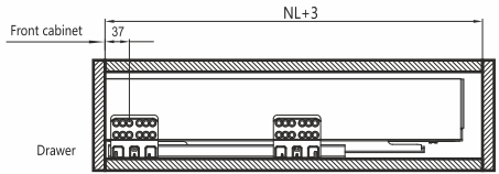
Cutting Dimensions for 16mm - thick MDF
