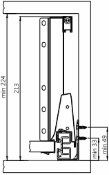
Cabinet Space Requirements
