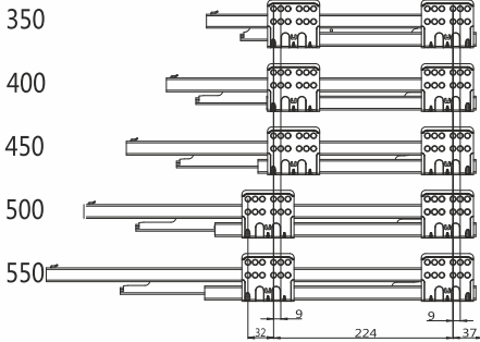
Cutting Dimensions for 16mm - thick MDF
