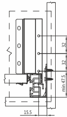
Front Connectors Panel Mounting dimension
